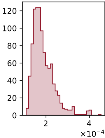
RL
