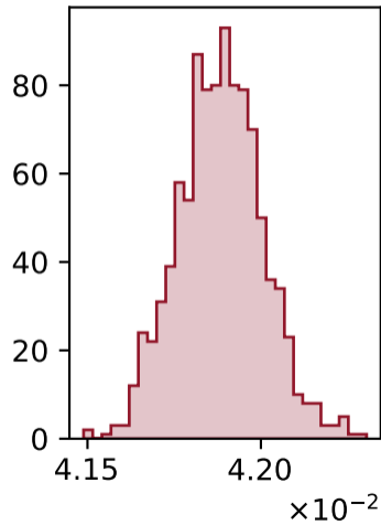
convolution
