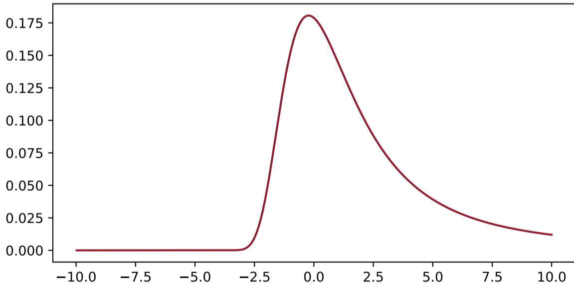
Landau distribution
