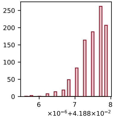
convolution
