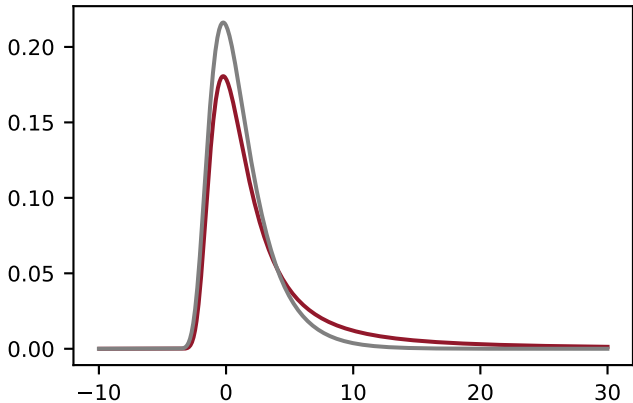
Landau distribution
