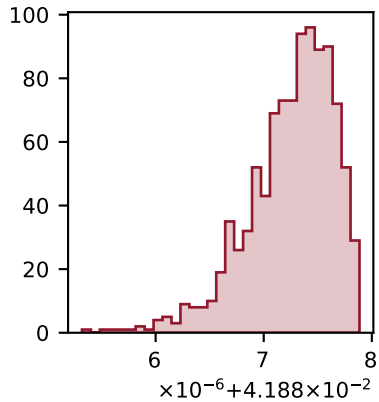
convolution
