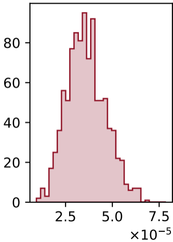
RL
