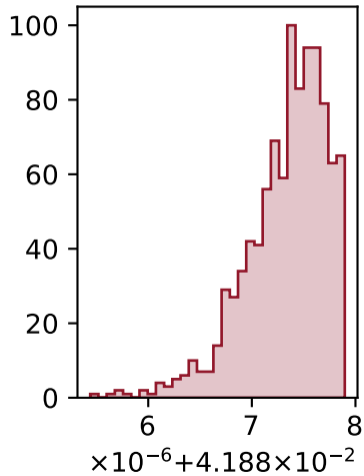
convolution
