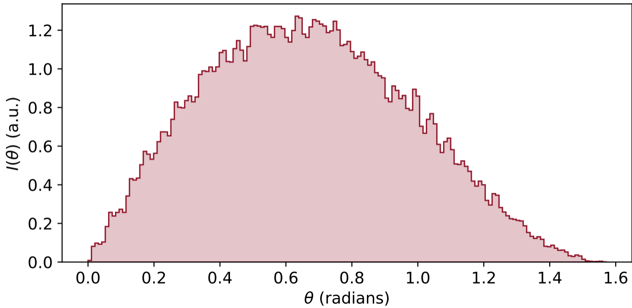
Deconvolved with RL at \sigma = 0.5
